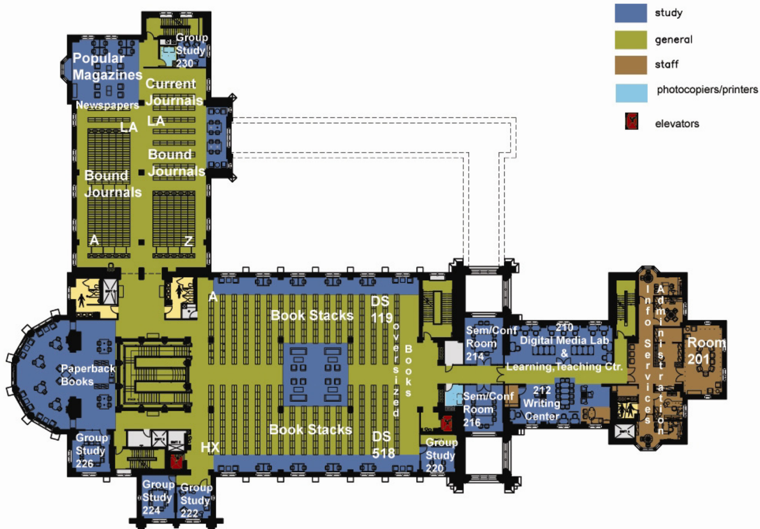
SECOND LEVEL FLOOR PLAN
