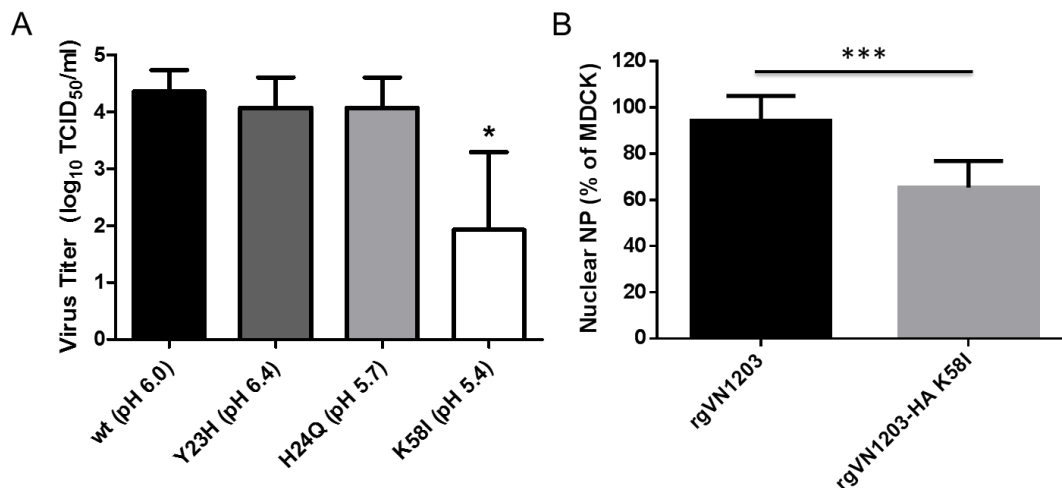
Figure 5: Destabilization of the H5 HA (more H1-like) reduces viral replication and nuclear entry in macrophages. (A) Raw264.7 macrophages were infected with wild-
